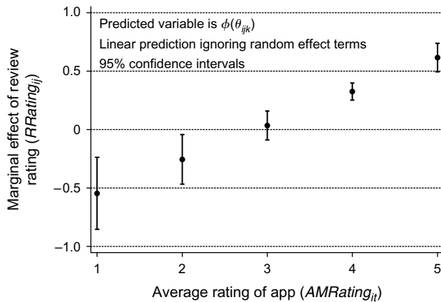
Figure 2 Marginal Effects in Vote-Level Analysis
