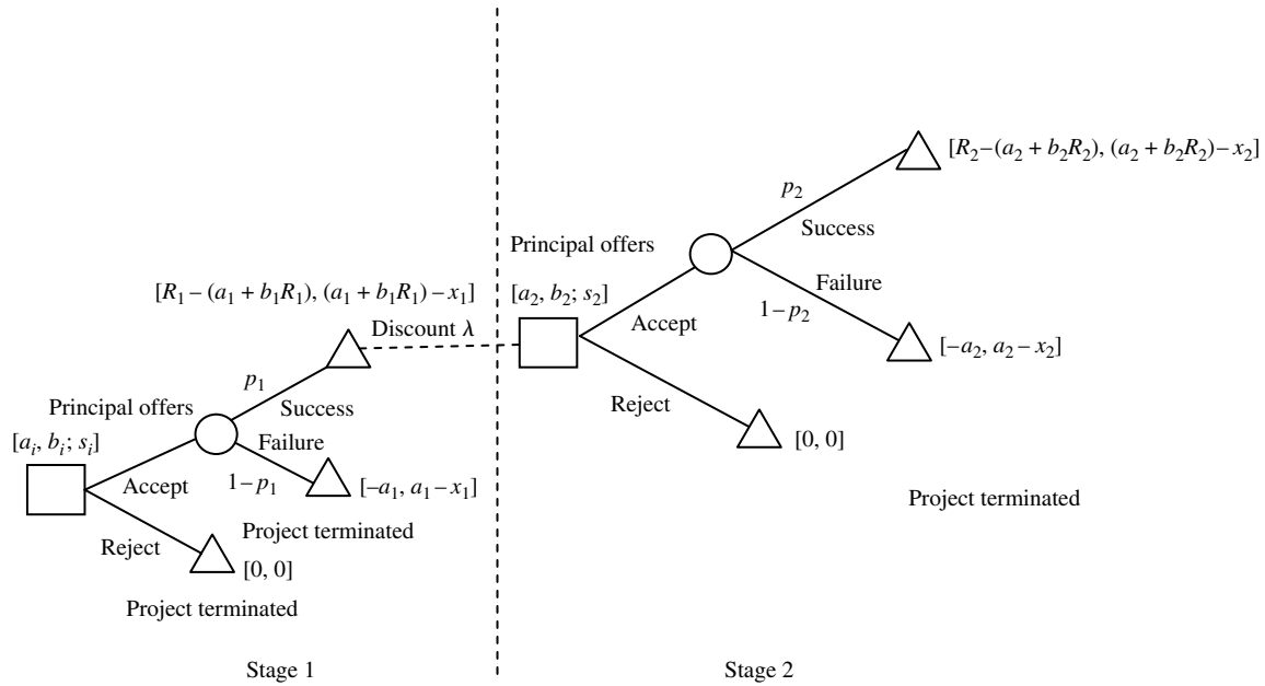
Figure 1 Decision Tree
