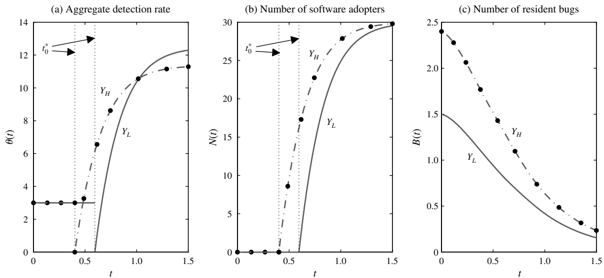
Figure 3 Optimal Release Time as Influenced by Changes in Software Functionality
