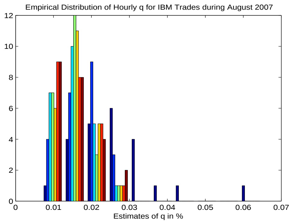
Figure 2: Empirical Distribution of Hourly q for IBM Trades during August 2007
