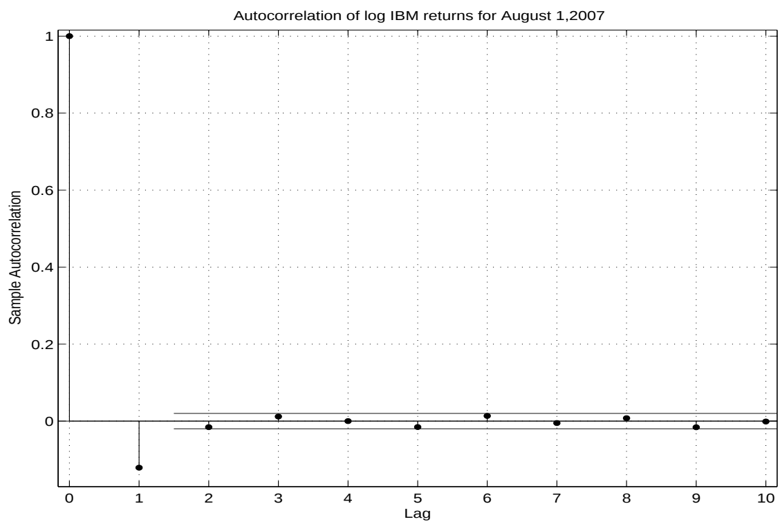
Figure 1: Sample Autocorrelation of IBM Stock Returns during August 2007
